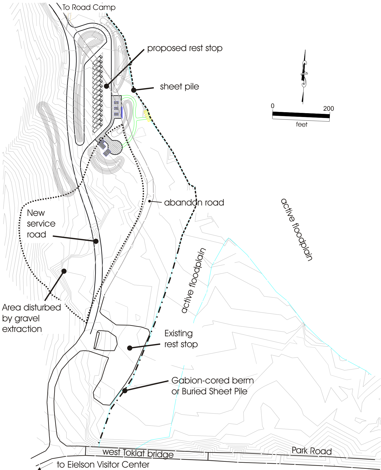
Figure 8 - Alternative 2 - Toklat Proposed Site Plan
