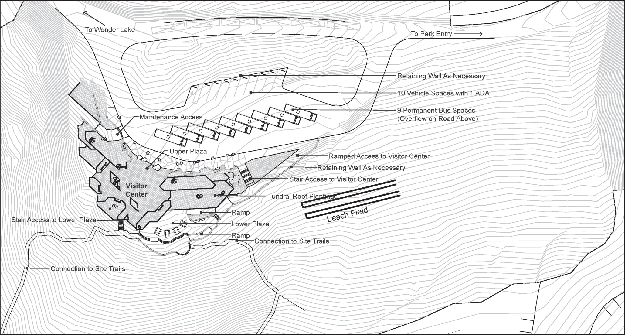
Figure 4 Eielson Visitor Center - Proposed Site Plan
