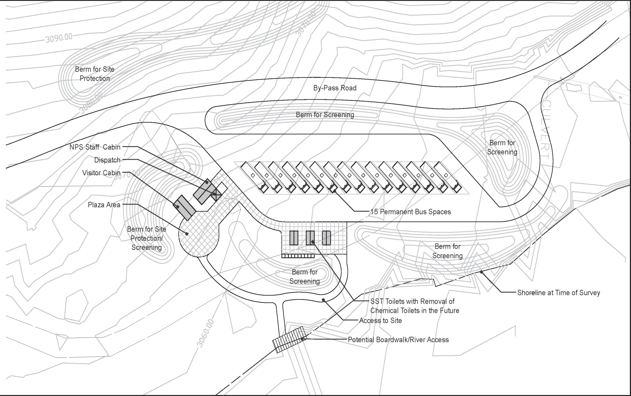
Figure 7 - Toklat Conformed Schematic Design
