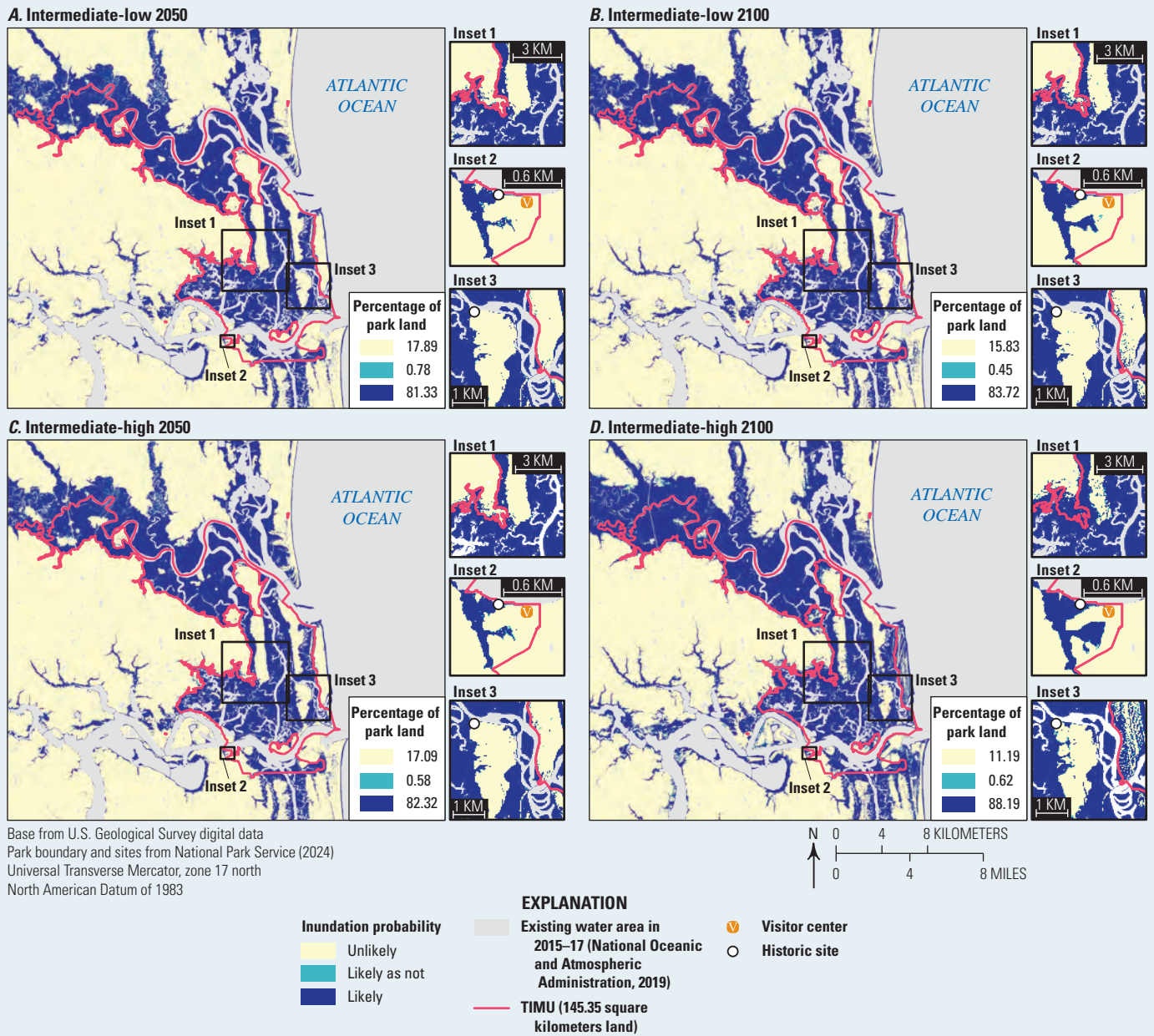
Figure 4. Sea-level rise (SLR) inundation probabilities for Timucuan Ecological and Historic Preserve (TIMU), Florida, under the SLR scenarios (Sweet and others, 2022) intermediate-low for the years A , 2050 and B , 2100 and intermediate-high for the years C , 2050 and D , 2100 (Thurman and others, 2024). Sea-level change projected in this figure is relative to the year 1992. Probability is shown using three bins developed for the Intergovernmental Panel on Climate Change (2022): unlikely, probability less than or equal to 0.33; likely as not, probability greater than 0.33 and less than or equal to 0.66; and likely, probability greater than 0.66. Existing water areas were excluded from the analyses and area calculations; KM, kilometer.
