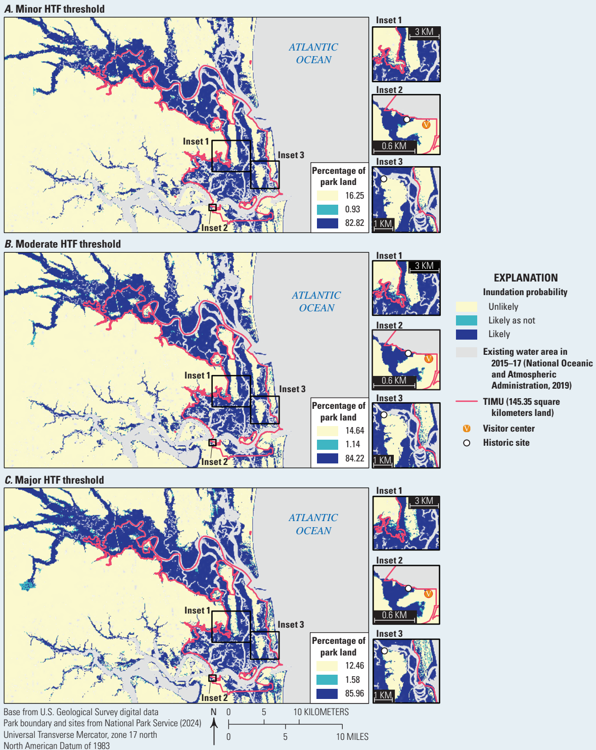
Figure 5. High tide flooding (HTF) inundation probabilities for Timucuan Ecological and Historic Preserve (TIMU), Florida, under the National Oceanic and Atmospheric Administration (Sweet and others, 2022) A , minor, B , moderate, and C , major HTF thresholds (Thurman and others, 2024). Probability is shown using three bins developed for the Intergovernmental Panel on Climate Change (2022): unlikely, probability less than or equal to 0.33; likely as not, probability greater than 0.33 and less than or equal to 0.66; and likely, probability greater than 0.66. Existing water areas were excluded from the analyses and area calculations; KM, kilometer.
