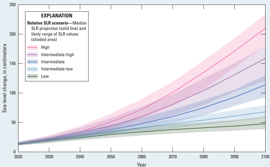
Figure 2. Relative sea-level rise (SLR) scenarios for Timucuan Ecological and Historic Preserve (TIMU), Florida, associated with the five global SLR scenarios from Sweet and others (2022). Sea-level change projected in this figure (modified from Thurman and others [2024]) is relative to the year 1992.
