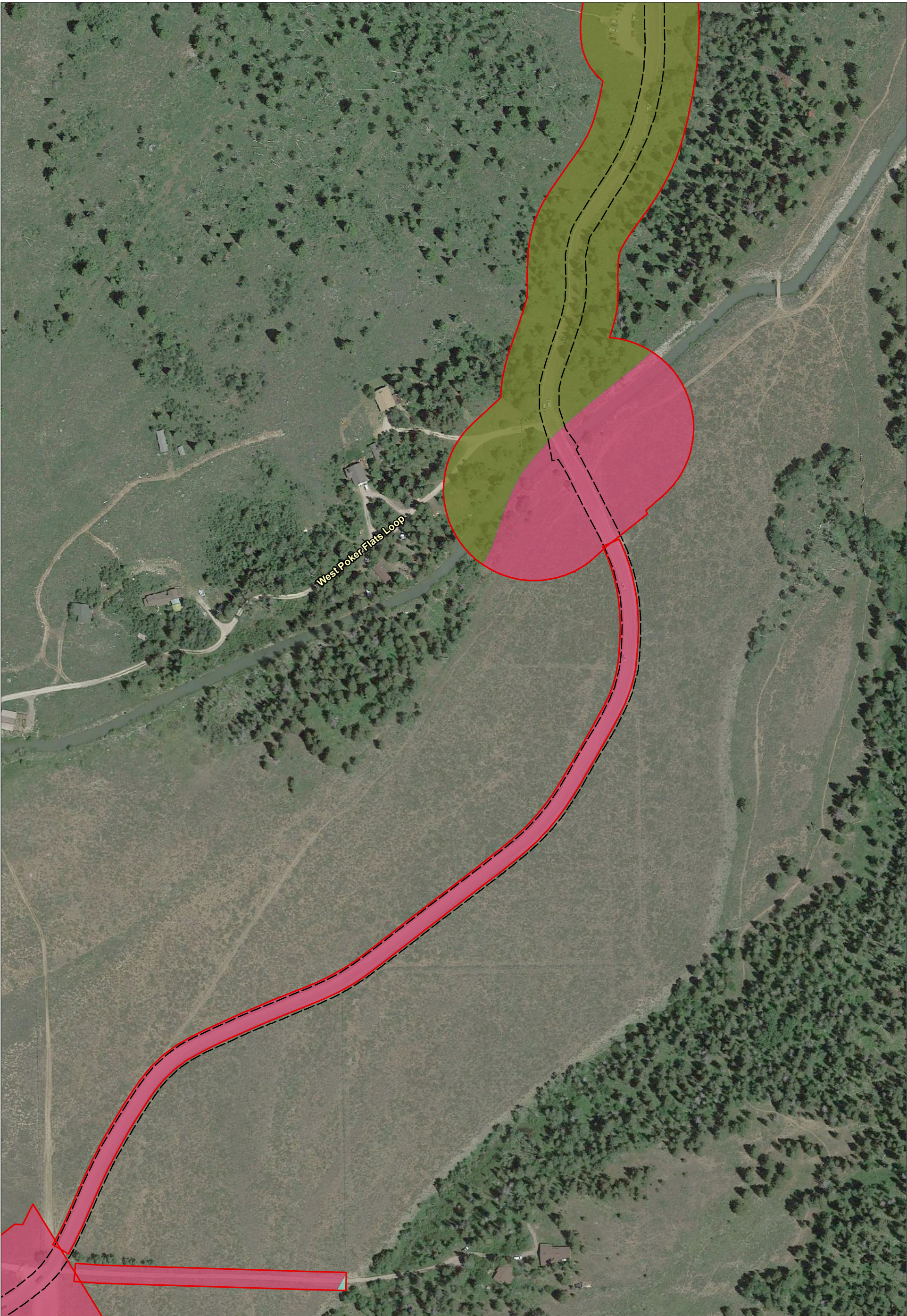
Figure 2 Soils
