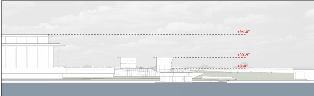
Figure 12: Alternative C1 – Two Land-Based Pavilions Plus River Pavilion with At-Grade Crossing, section showing relative heights of existing building and pavilions.
