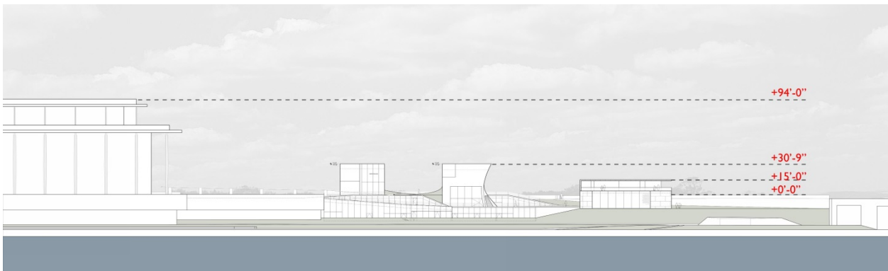
Figure 10: Alternative B – Three Land-Based Pavilions, section showing relative heights of existing building and pavilions.
